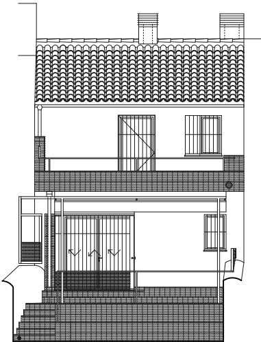
ALZADO INTERIOR
